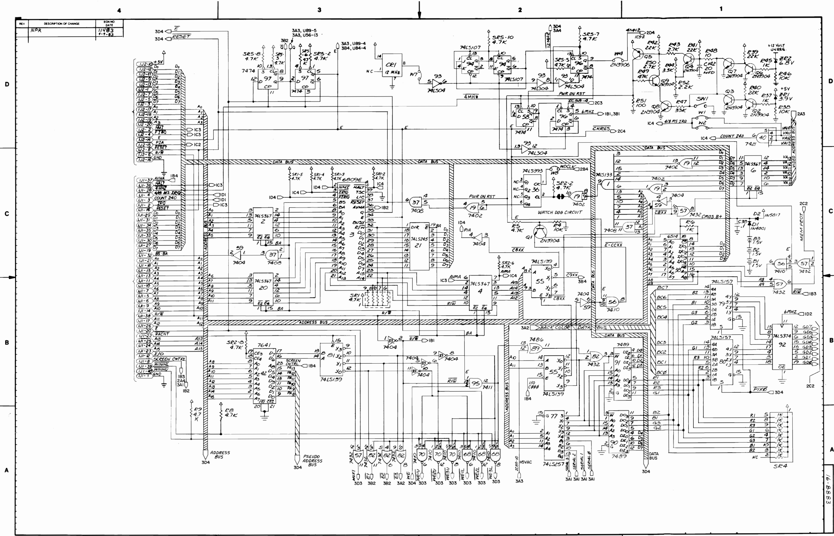
CPU Board Logic Diagram (Sheet 1 of 3)
