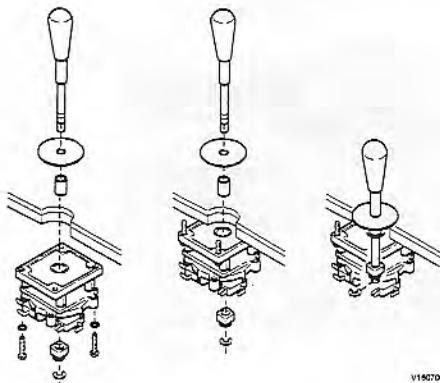
Figure 5: Joystick Installation
