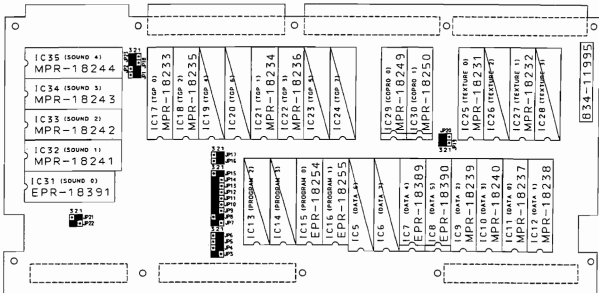
FIGURE 42: ROM BOARD
