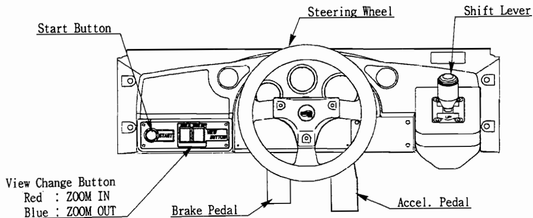
FIGURE 18: CONTROL LOCATIONS
