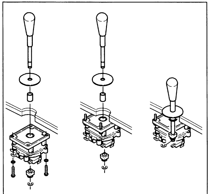
FIGURE 4 Joystick Installation
