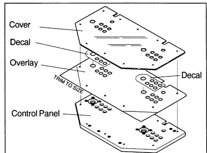
FIGURE 1 Overlay Installation
