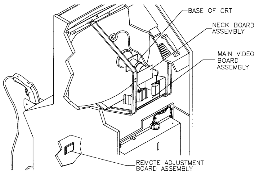
Cutaway Rear View
