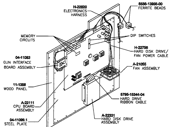
Interior View of Electronics
