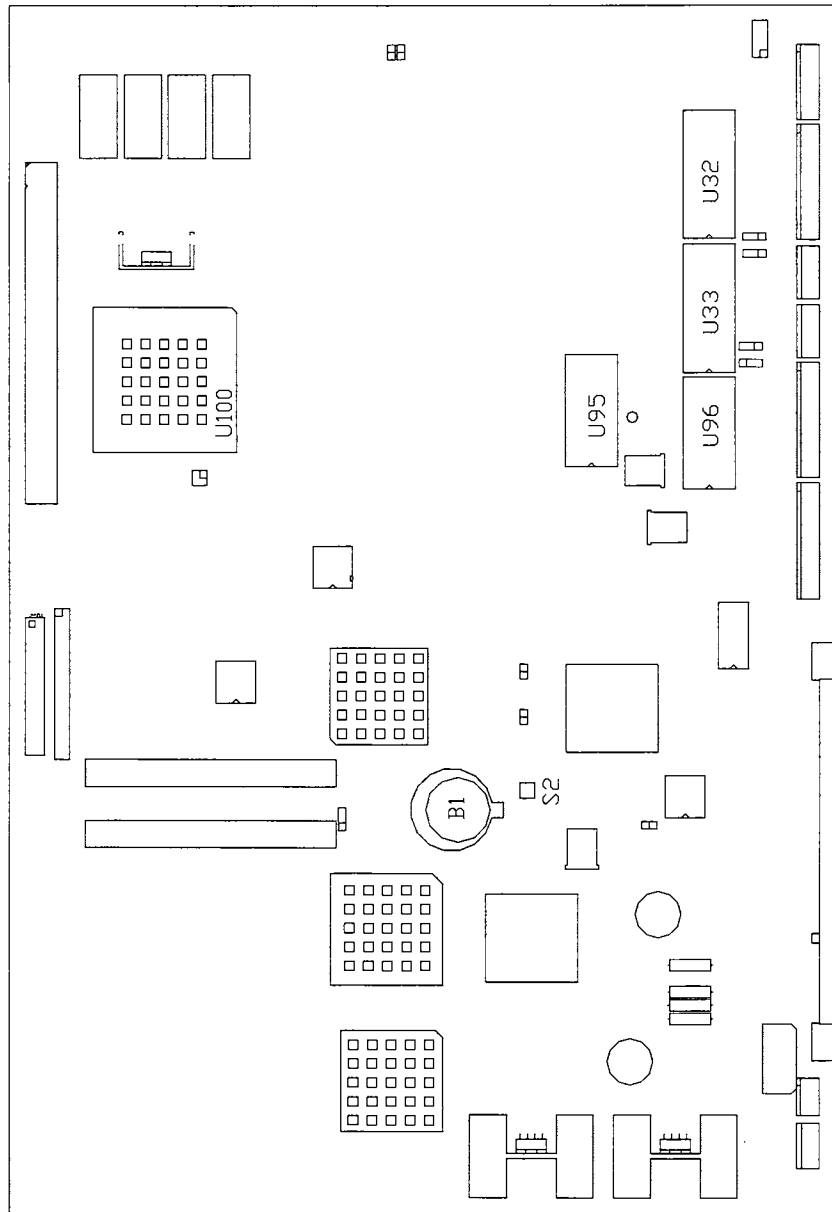
INDICATOR, SWITCH AND JUMPER LOCATIONS
