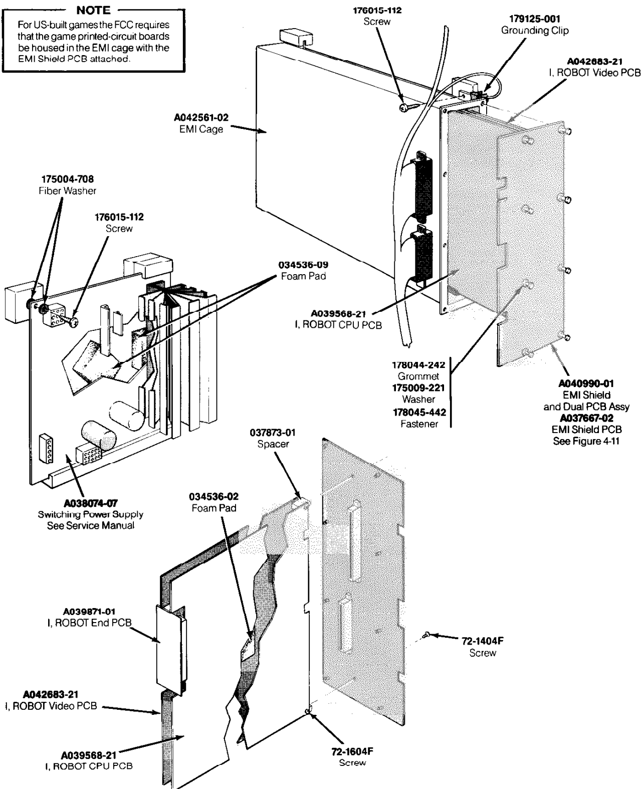
Figure 4-8 Printed-Circuit Board Mounting Hardware (US & Ireland)
