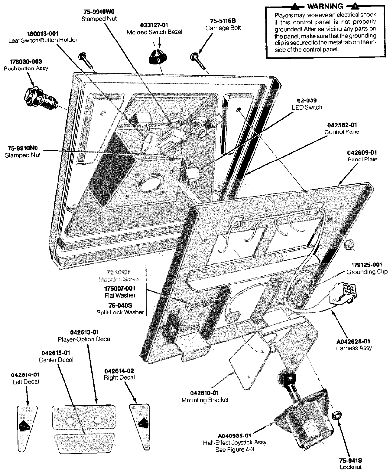
Figure 4-2 Control Panel Assembly A042603-01 A
