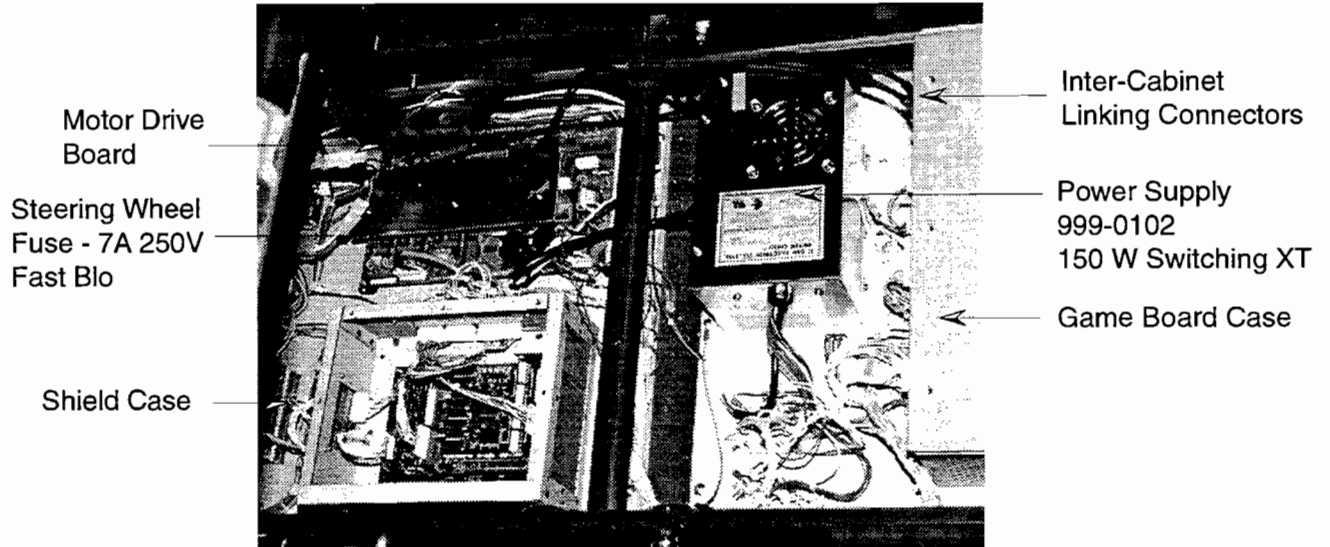
FIGURE 47: SHIELD CASE AND FUSE LOCATIONS - UNDER MIDDLE FLOORBOARD
