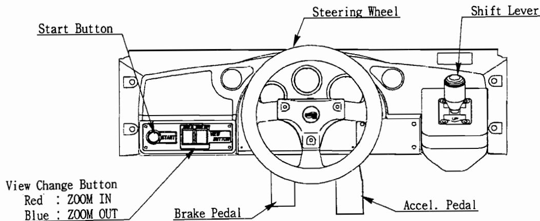
FIGURE 18: CONTROL LOCATIONS
