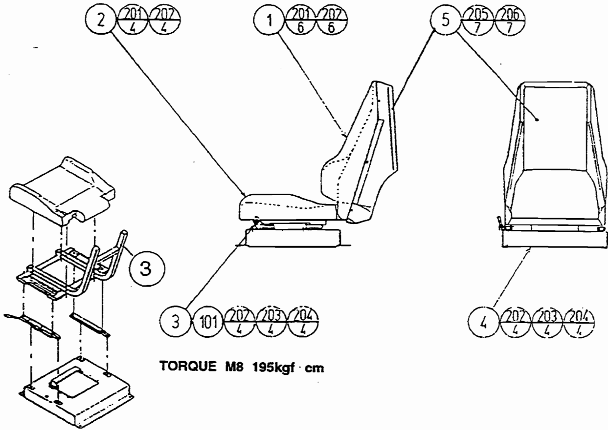
FIGURE 40: SEAT ASSEMBLY
