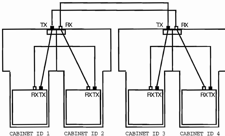
FIGURE 23: FOUR PLAYER LINKING DIAGRAM
