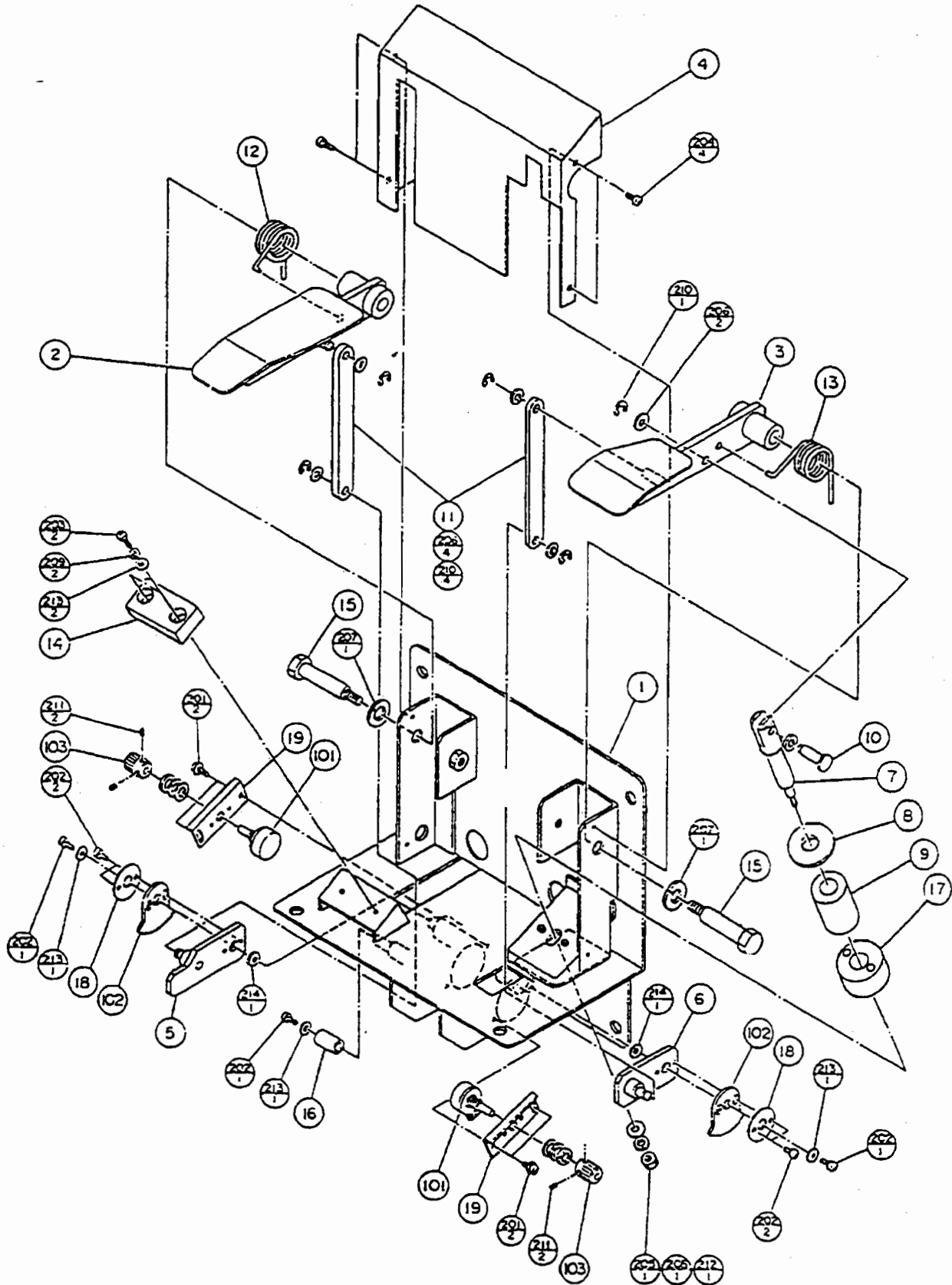
FIGURE 39: GAS AND BRAKE PEDAL ASSEMBLY
