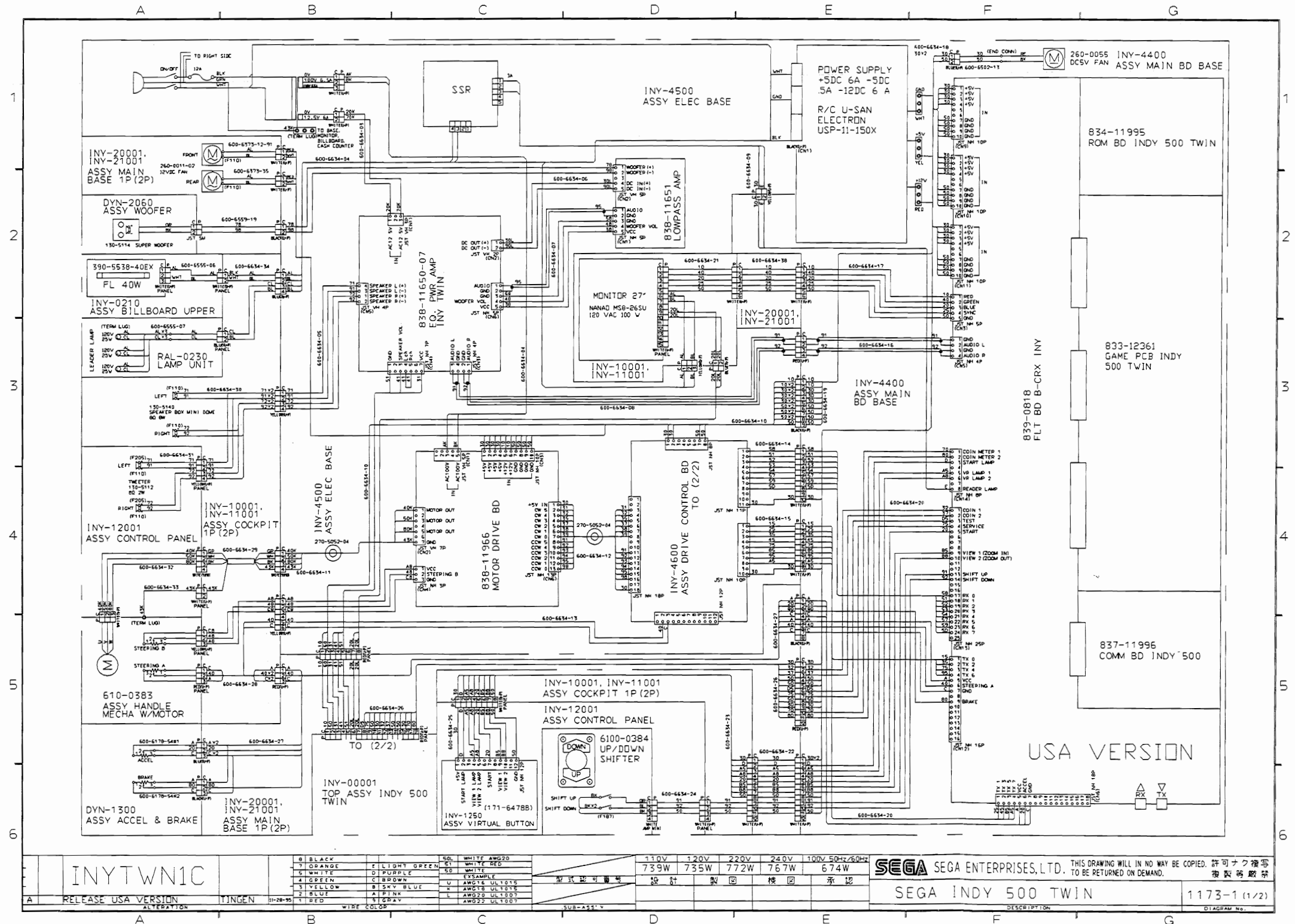
FIGURE 68: INDY 500 TWIN WIRING DIAGRAM - PAGE 1 OF 2
