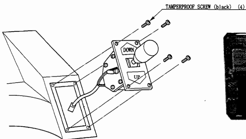
FIGURE 64: SHIFT LEVER ACCESS
