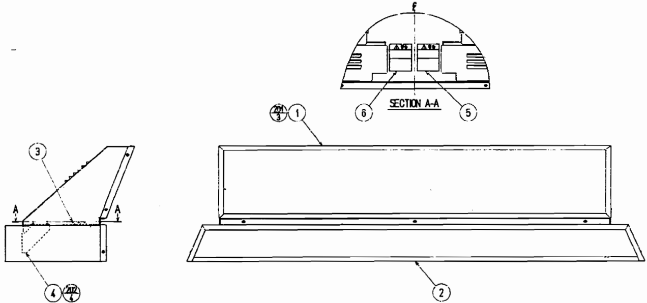
FIGURE 32: BILLBOARD ASSEMBLY
