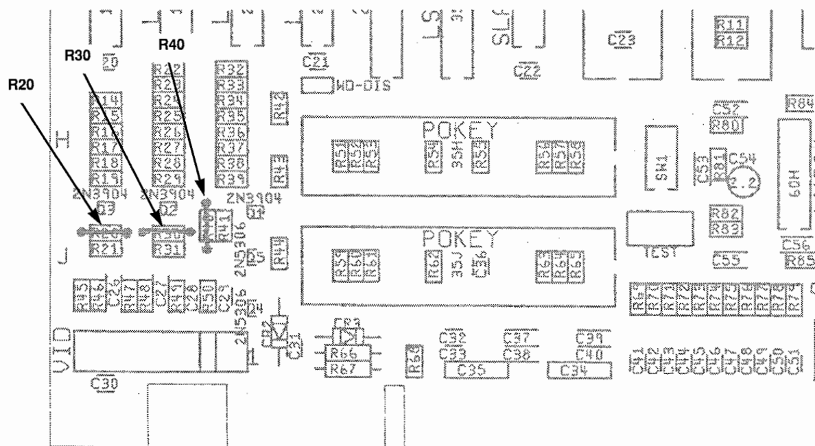
Figure 3-1 Shorting Out Resistors on Tetris Game PCB
