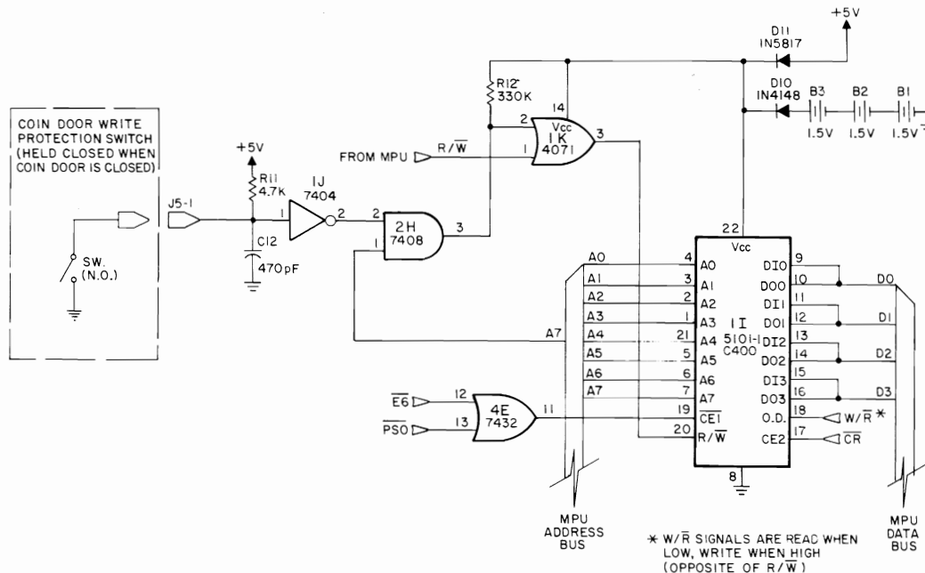
Figure 3-16. CMOS RAM
