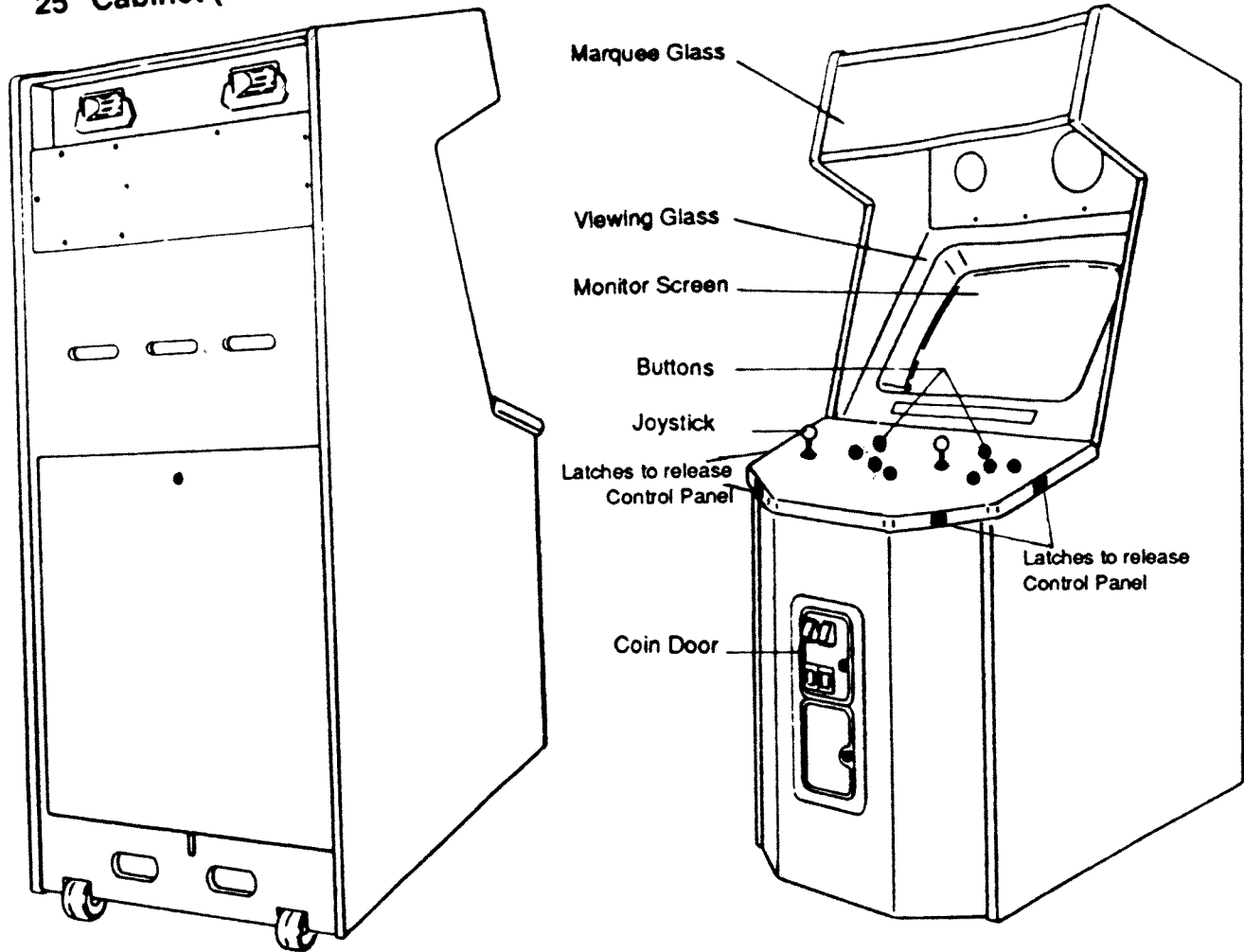
Cabinet Assembly
