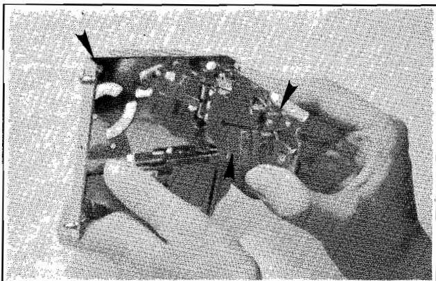
Figure 3-4 Surfaces to Clean Inside the Coin Mechanism
