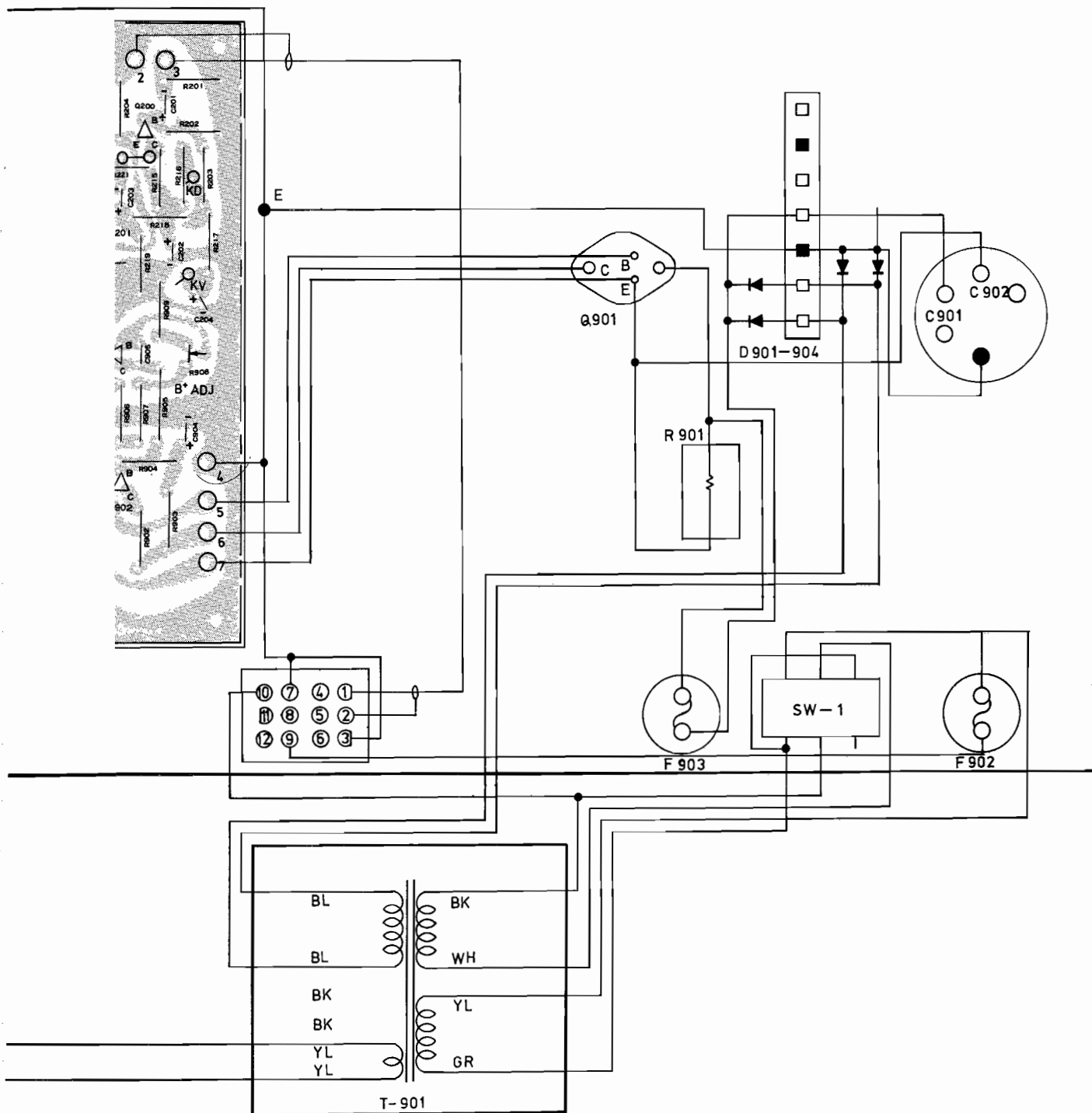
BOTTOM VIEW
