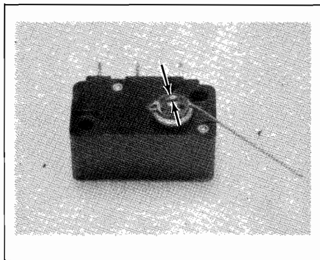
Figure 3-8 Securing the Coin Switch Trip Wire
