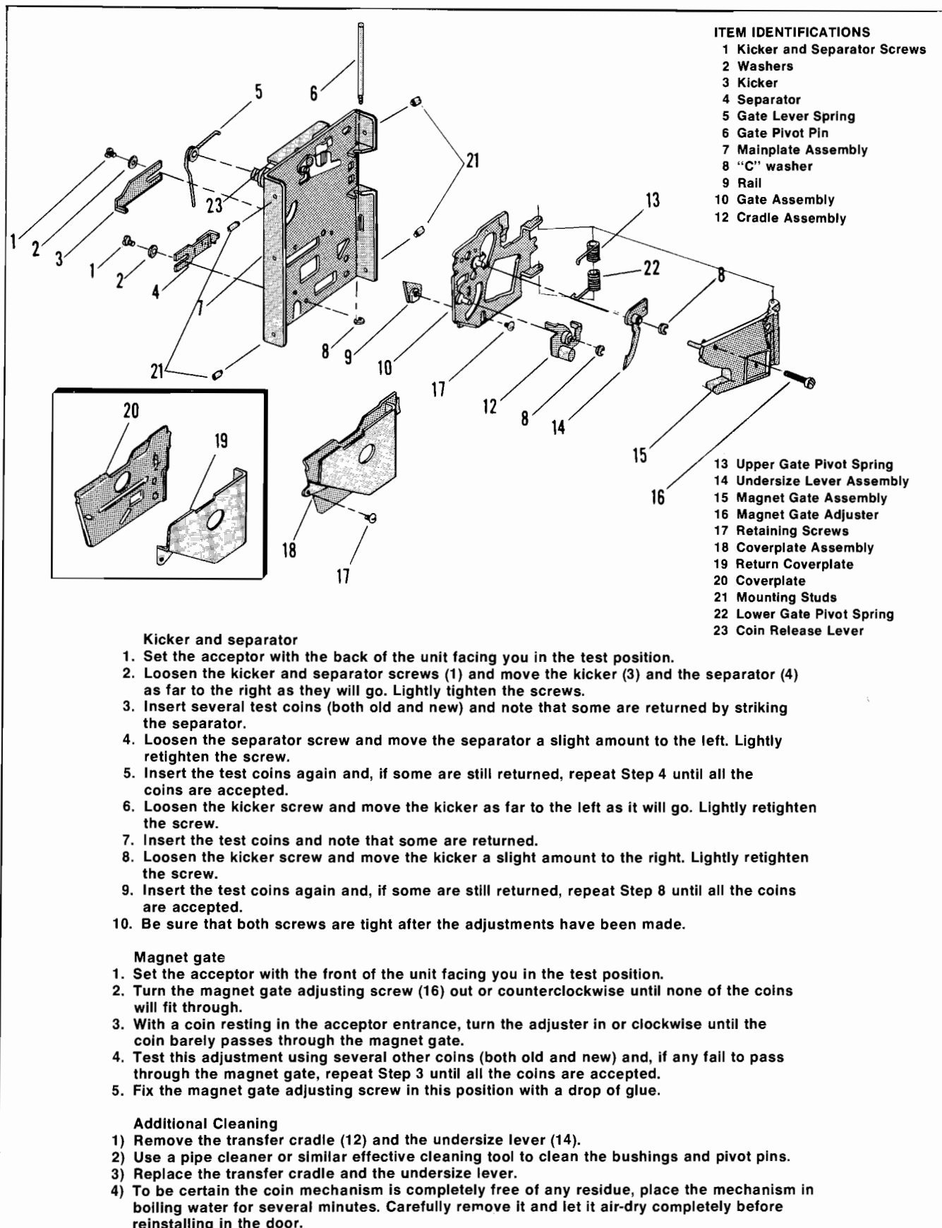
Figure 3-9 Adjustments on Coin Mechanism
