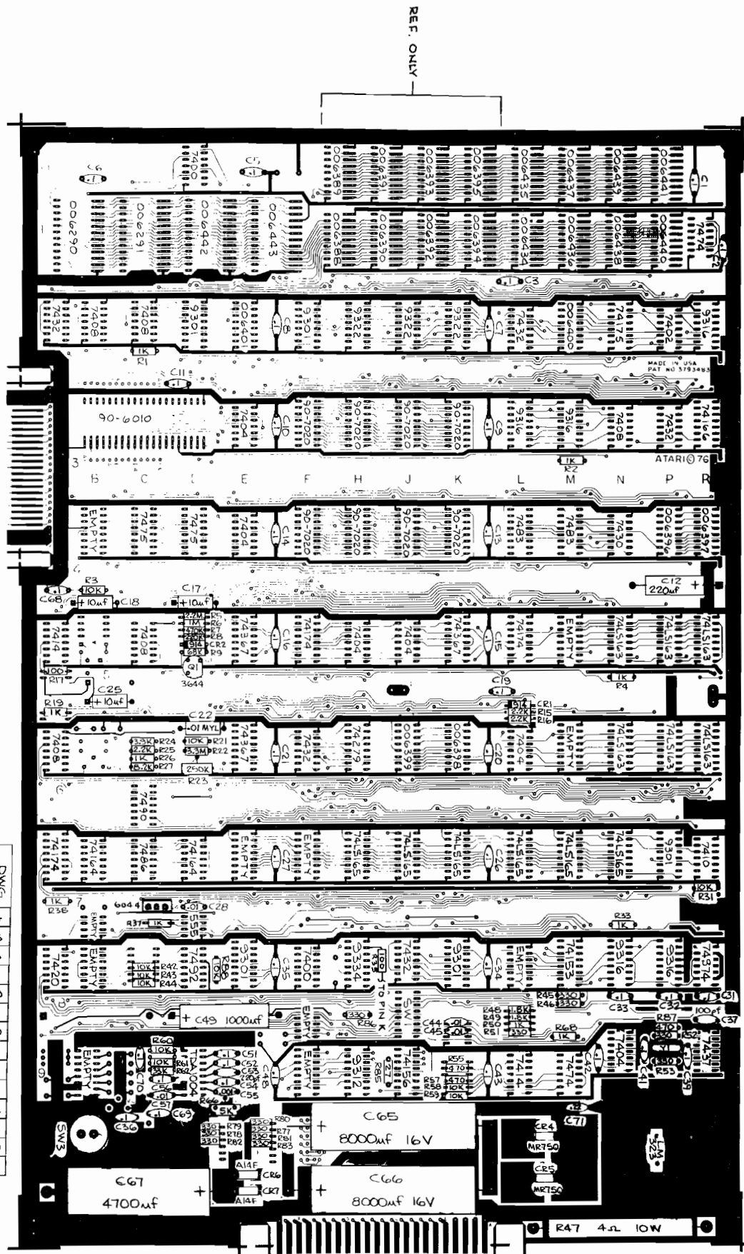
Figure 5-12 Sprint One PCB Assembly A006433-01 and -02 C
