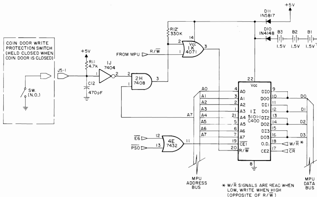
Figure 3-16. CMOS RAM
