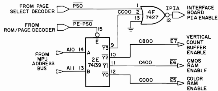
Figure 3-15. Page 0 Decoder
