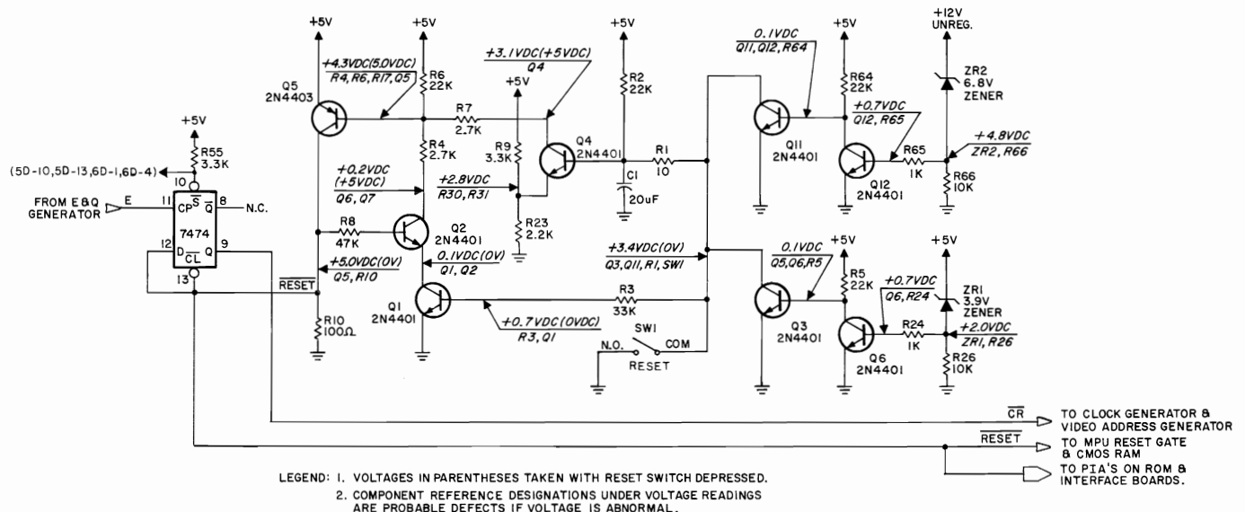
Figure 3-1. Reset Circuit
