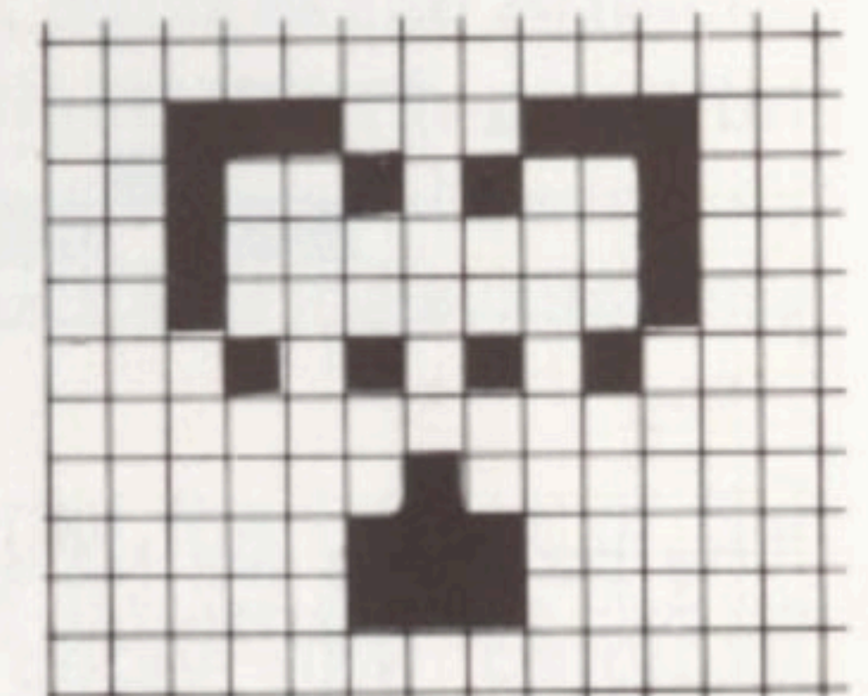
Puffer train #2
