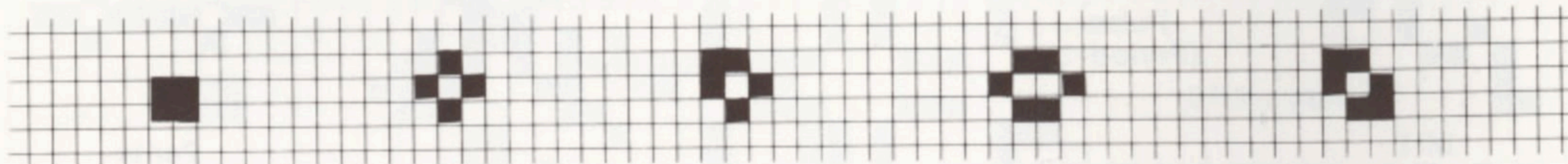
Ship
