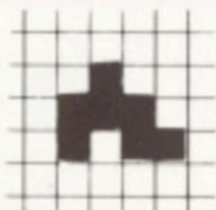
B heptomino
