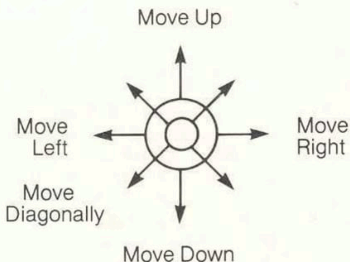
Figure 6 - Joystick Moves
