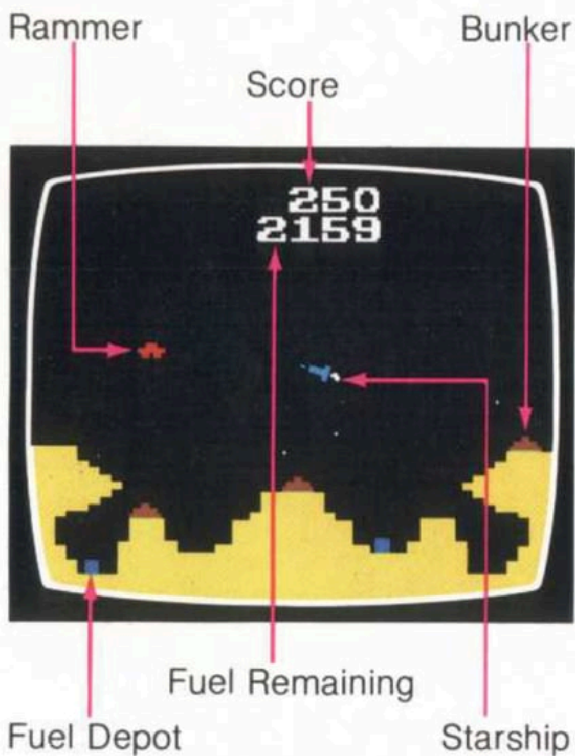
Figure 2—Planet Landscape
