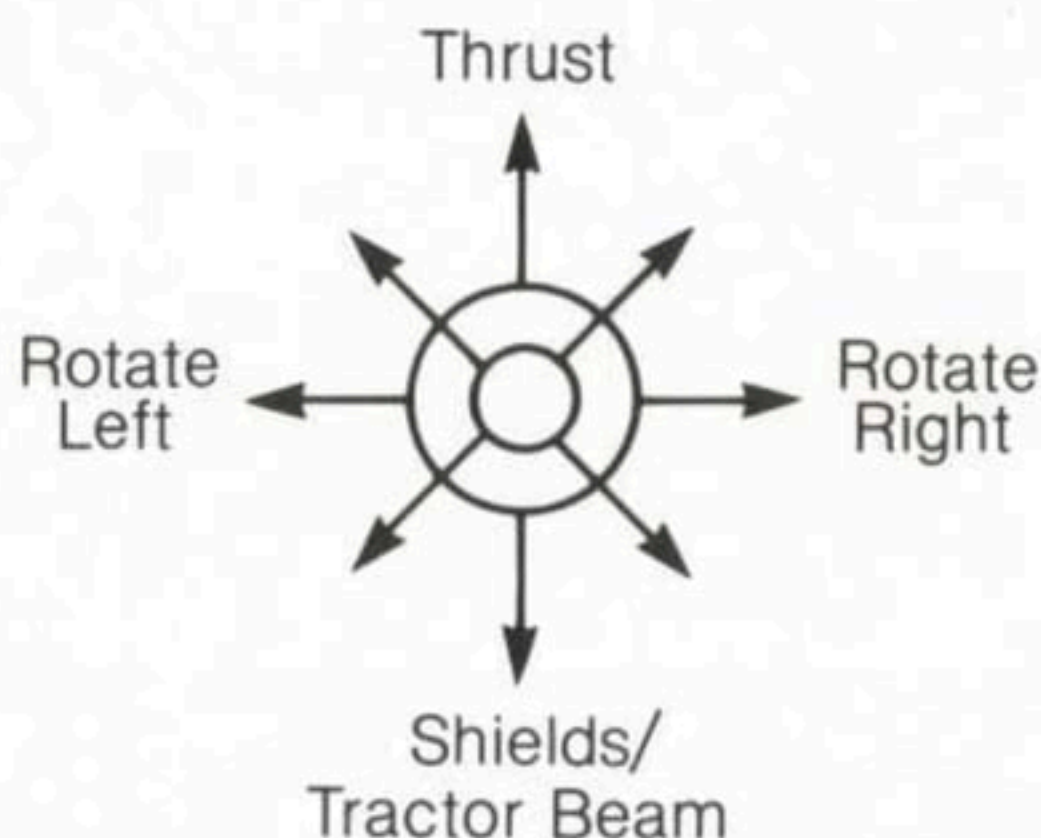
Figure 4—Spaceship Maneuvers
