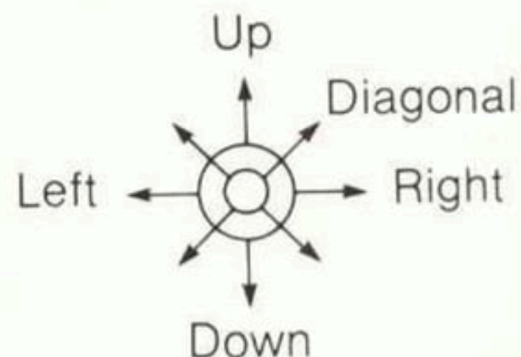
Figure 10 - Spaceship Moves
