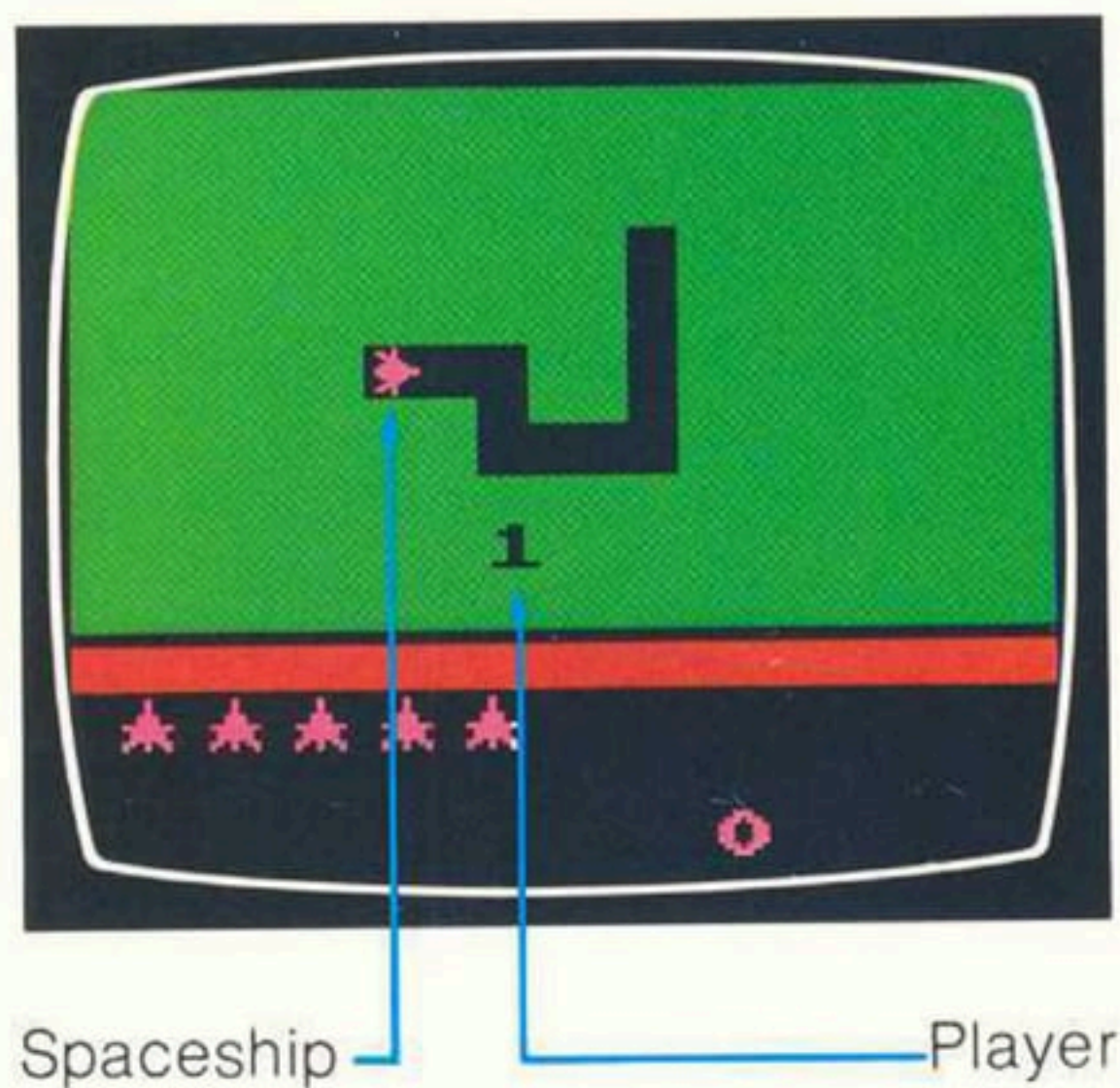
Figure 1 - Tunnel Map
