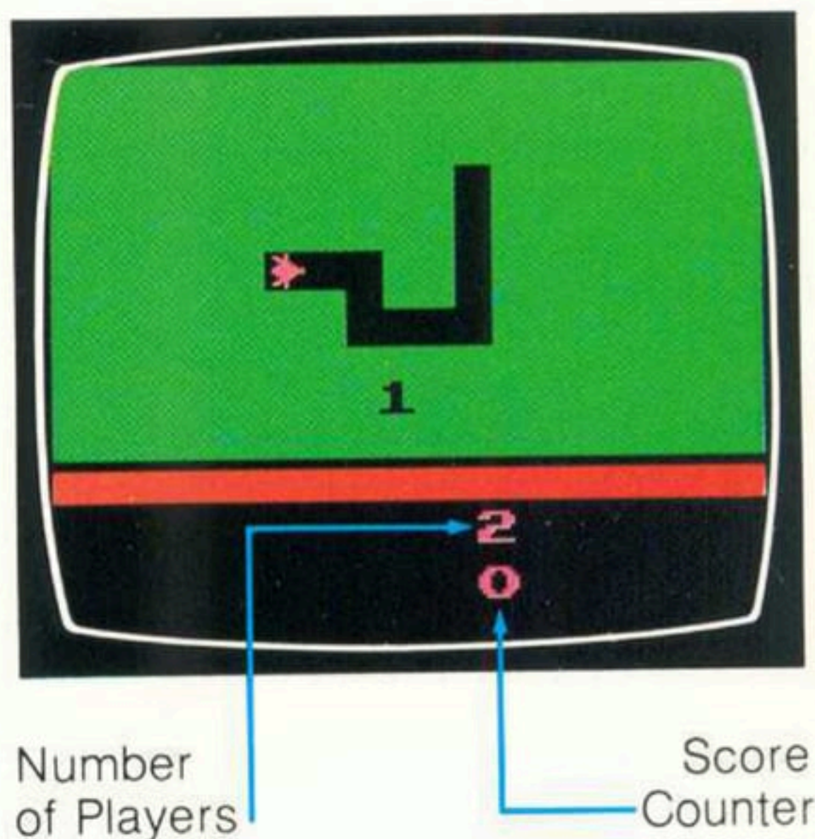
Figure 9 - Game Selection
