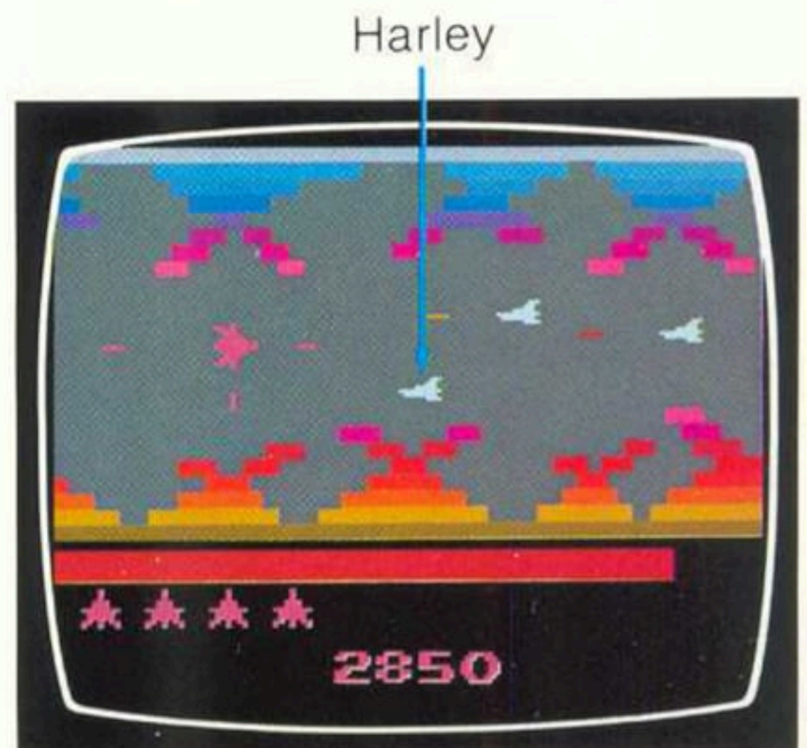
Figure 4 - Stick Zone
