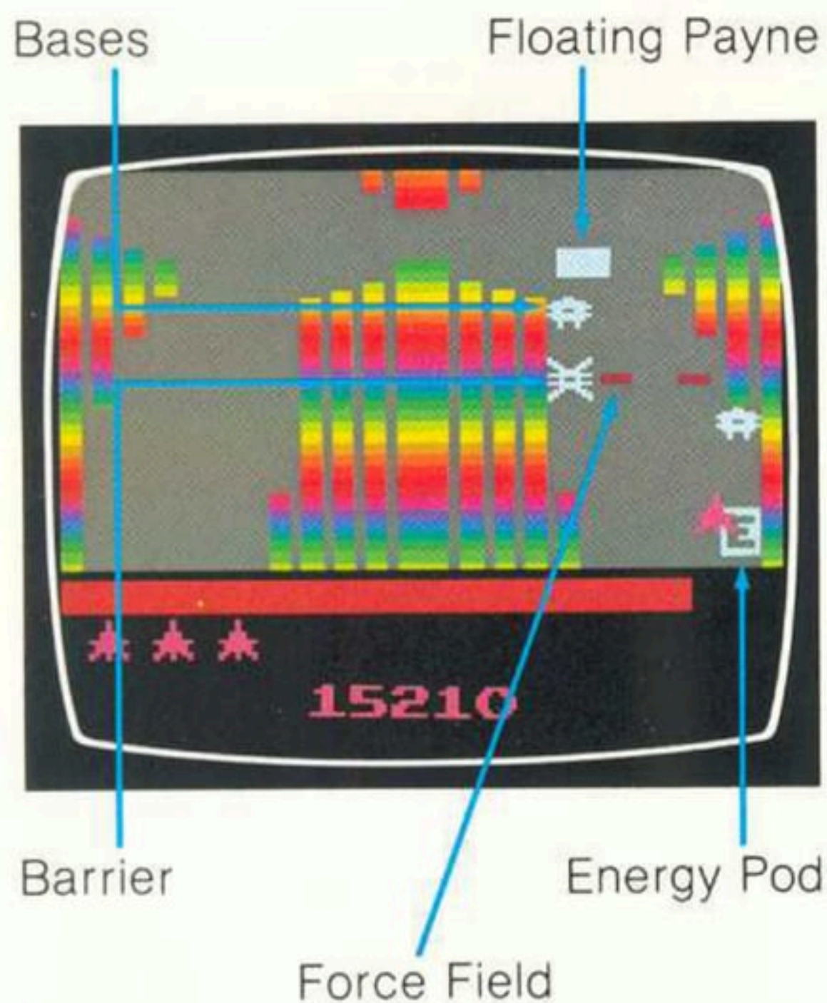
Figure 5 - Striped Zone
