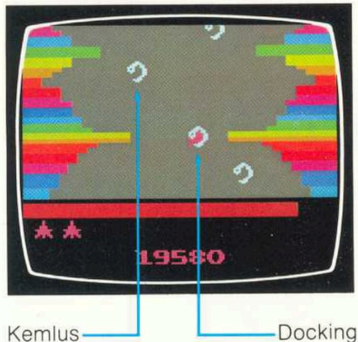
Figure 6 - Bleak Zone
