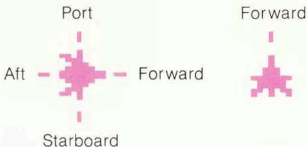
Figure 11 - Laser Fire
