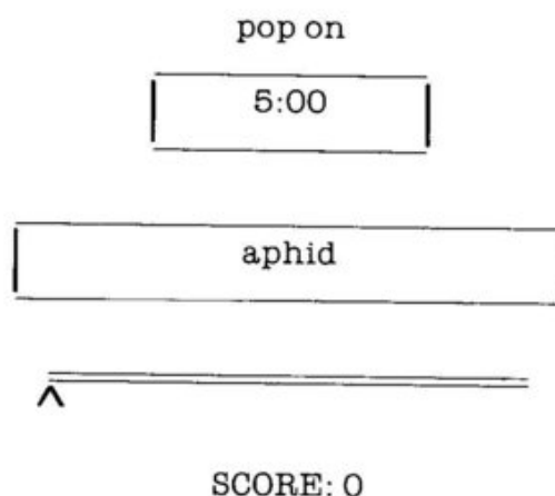
Figure 5 Pop On display screen
