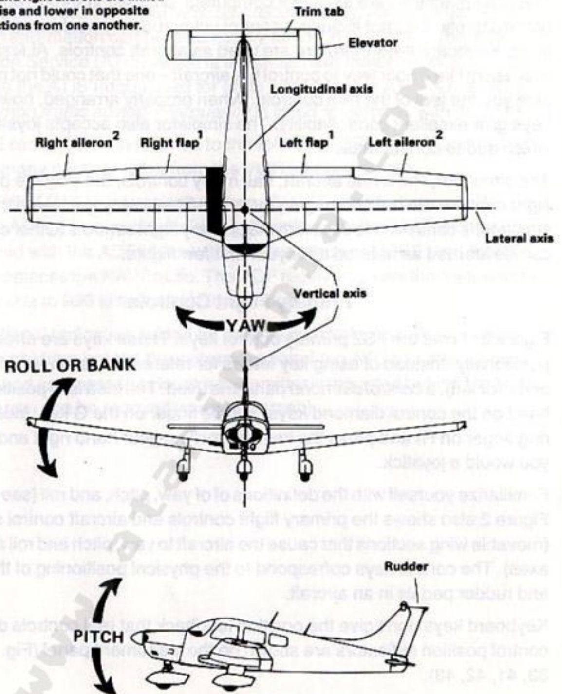
a) Control surfaces and rotational axes
