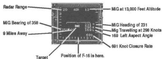
Tracking View Radar (20 mile range)
