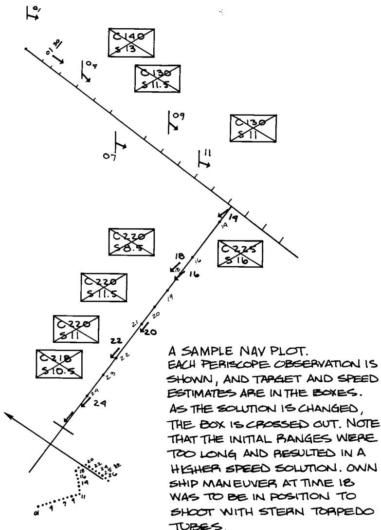
Figure 37. The navigational plot
