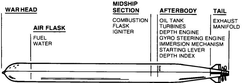
Figure 2. Typical torpedo design
