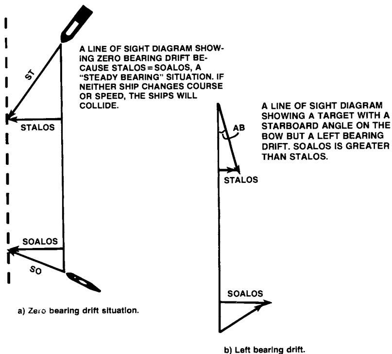
Figure 33. Bearing drift and steady bearing
