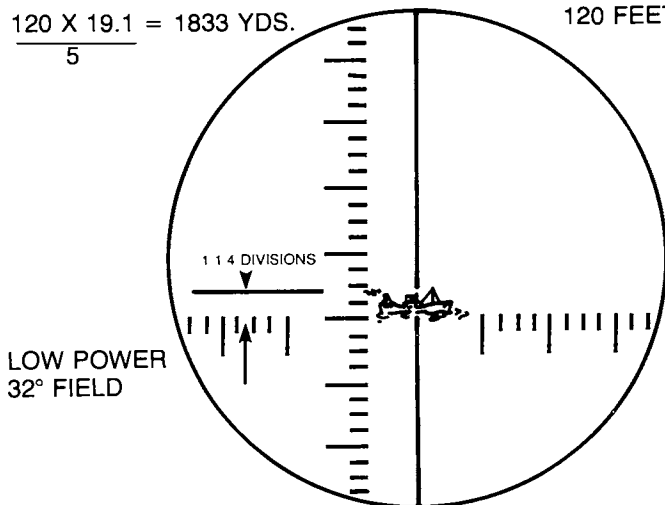
Figure 35. Telemeter ranging
