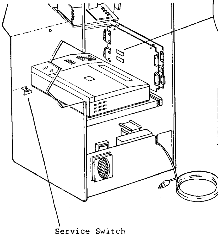
OPTION SWITCHES, SERVICE SWITCH
