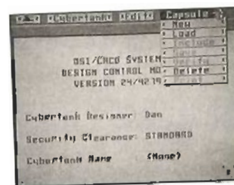
Diagram 2.2.3 --CAPSULE Menu
