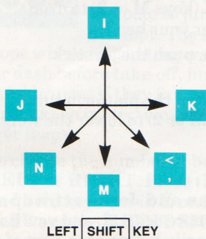
Keyboard Controls:
