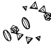
Tetrahedron
