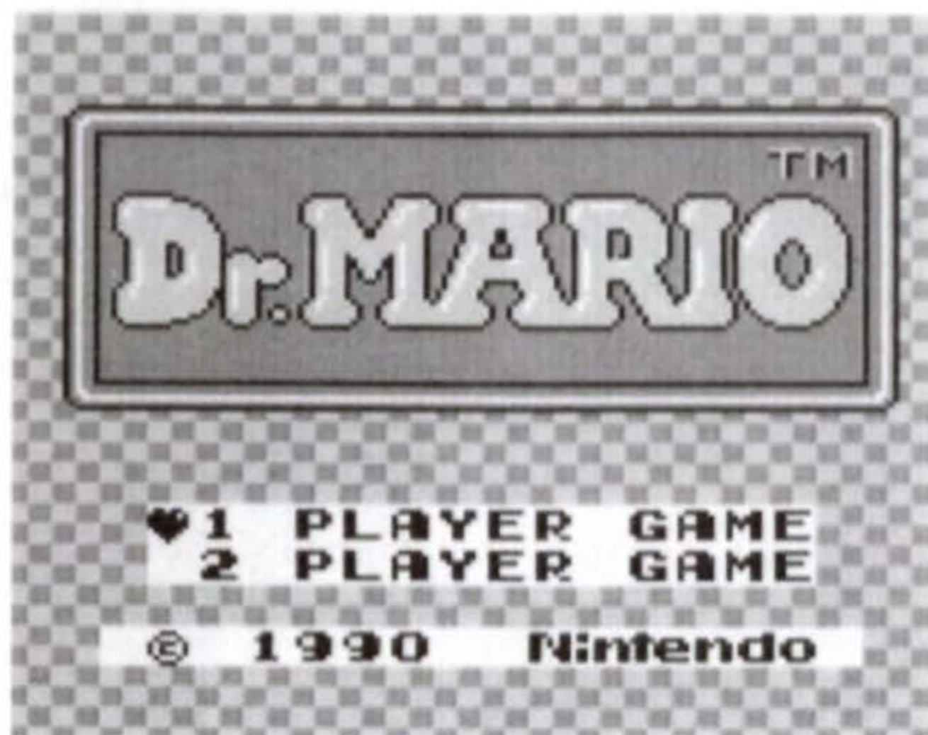
Menu Screen
