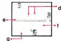
*Game screen
