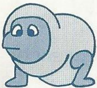
Fukuro- tokage
