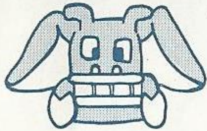
Biggs
